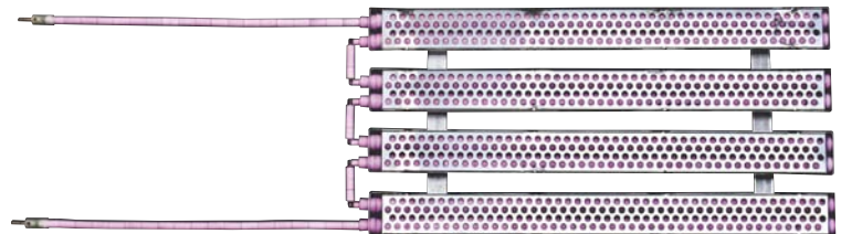
Channel Heater, 13kW, 240V
